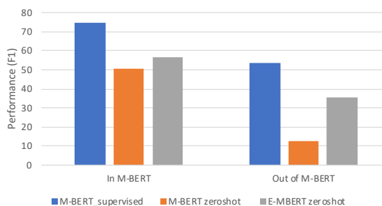
Figure 1: Comparison between M-BERT and our proposed approach E-MBERT: We report average zero-shot NER performance on 16 languages that are already in M-BERT and 11 new language that are out of M-BERT; M-BERT performance with supervised NER data is also reported as an upper-bound. In both languages in M-BERT and out of M-BERT, our method E-MBERT performs better than M-BERT.
